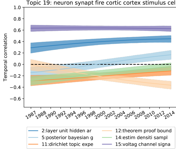
Figure 3: Evolution of the correlations between Topic 19 ( neuroscience ) and a few selected topics from DCTM. The solid line shows the 50th percentile and shaded area show the credible interval between 5th and 95th percentile. Topic 15 is consistently positively correlated with topic 19, which shares lots of similar words. The correlation with Topic 2 slowly increases over time. Instead, correlations with other topics are small and close to zero (dashed line), as they are mostly identified by disjoint sets of words.
