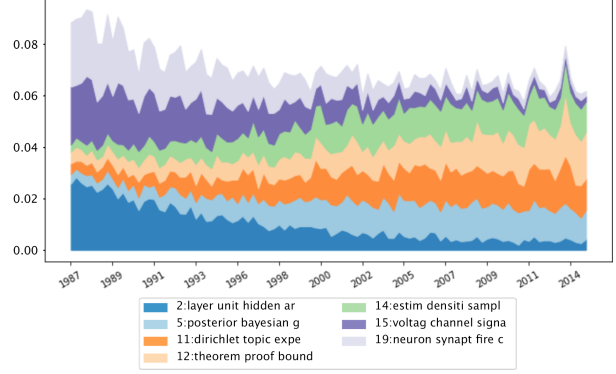
Figure 2: Evolution of the mean of the mixture of topics \sigma(\eta) for a few selected topics across the time span predicted from the trained DCTM. 2 Topics 15 and 19 are both associated with neuroscience , which exhibit a decreasing trend over time. Similarly there is a decreasing trend for neural networks after 1990.
