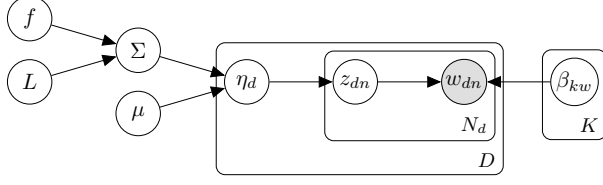
Figure 1: The graphical model for DCTM.
